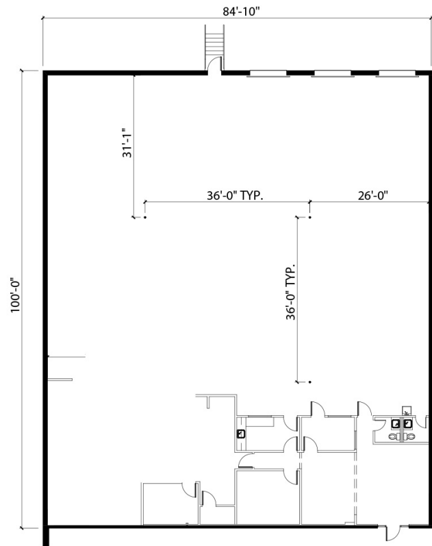
SUITE PLAN - 1/16" = 1'-0"
